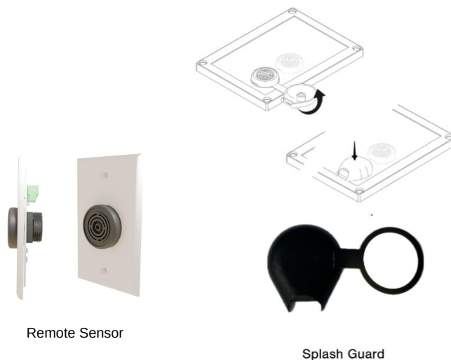
Splash Guard
